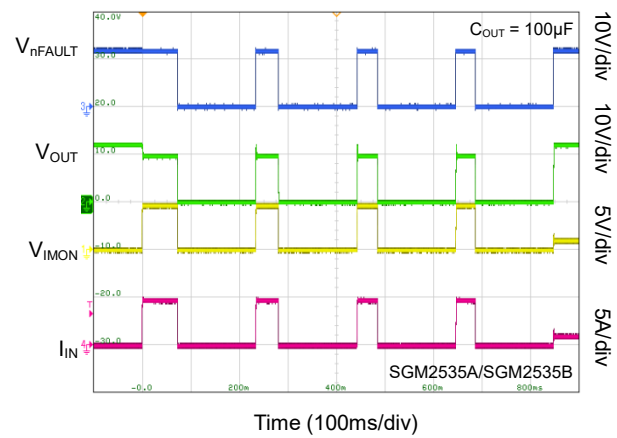
Overload Condition: Auto-Retry and Recovery
