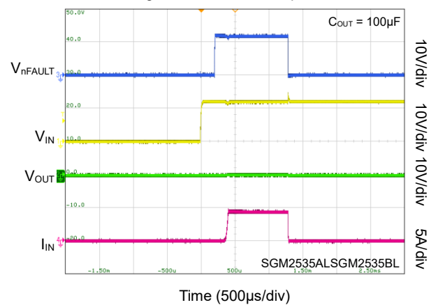
Hot Plug-In with Short on Output: Latched
