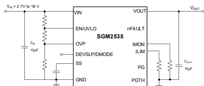
Figure 1. Simplified Schematic
