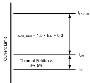
Figure 5. Fast-Trip Current
