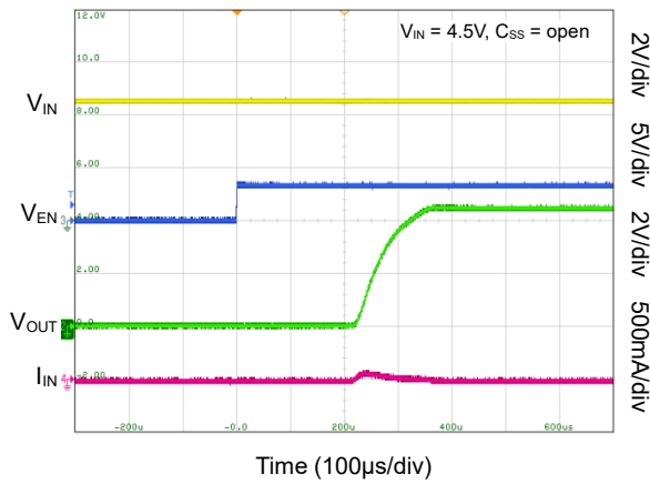
Turn-On with Enable
