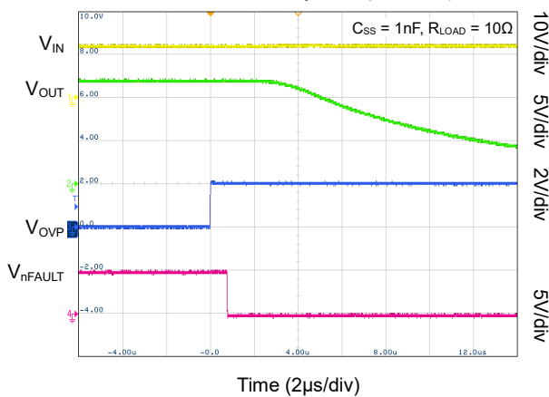
OVP Turn-Off Delay: OVP↑ to Fault↓
