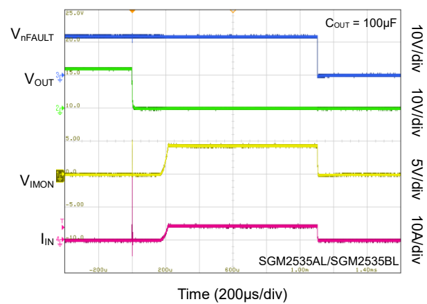
Hot-Short: Latched
