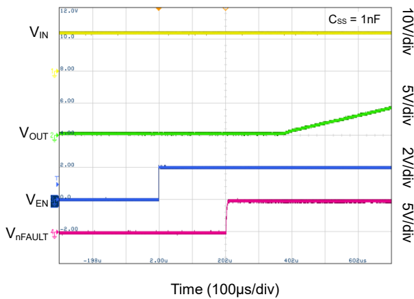
EN Turn-On Delay: EN↑ to Output Ramp↑
