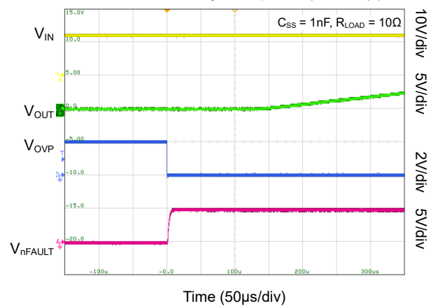
OVP Turn-On Delay: OVP↓ to Output Ramp↑
