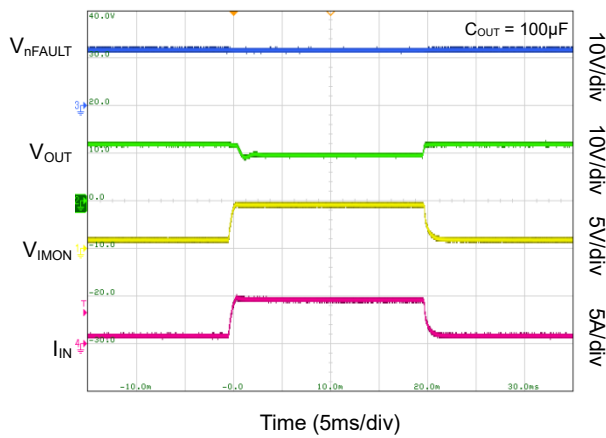
Overload: Step Change in Load from 12Ω to 2Ω and Back
