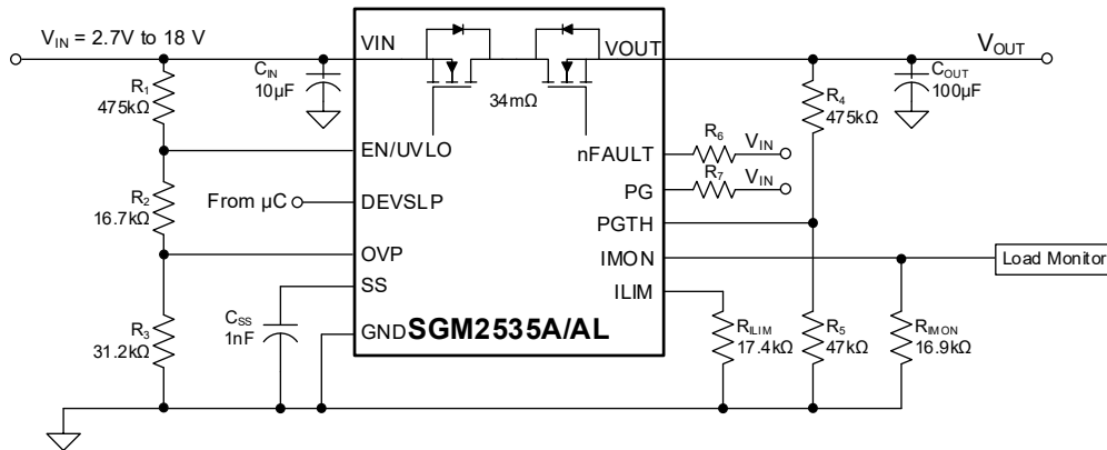
Figure 13. Typical Application Schematics: eFuse for Enterprise SSDs-SGM2535A/AL
