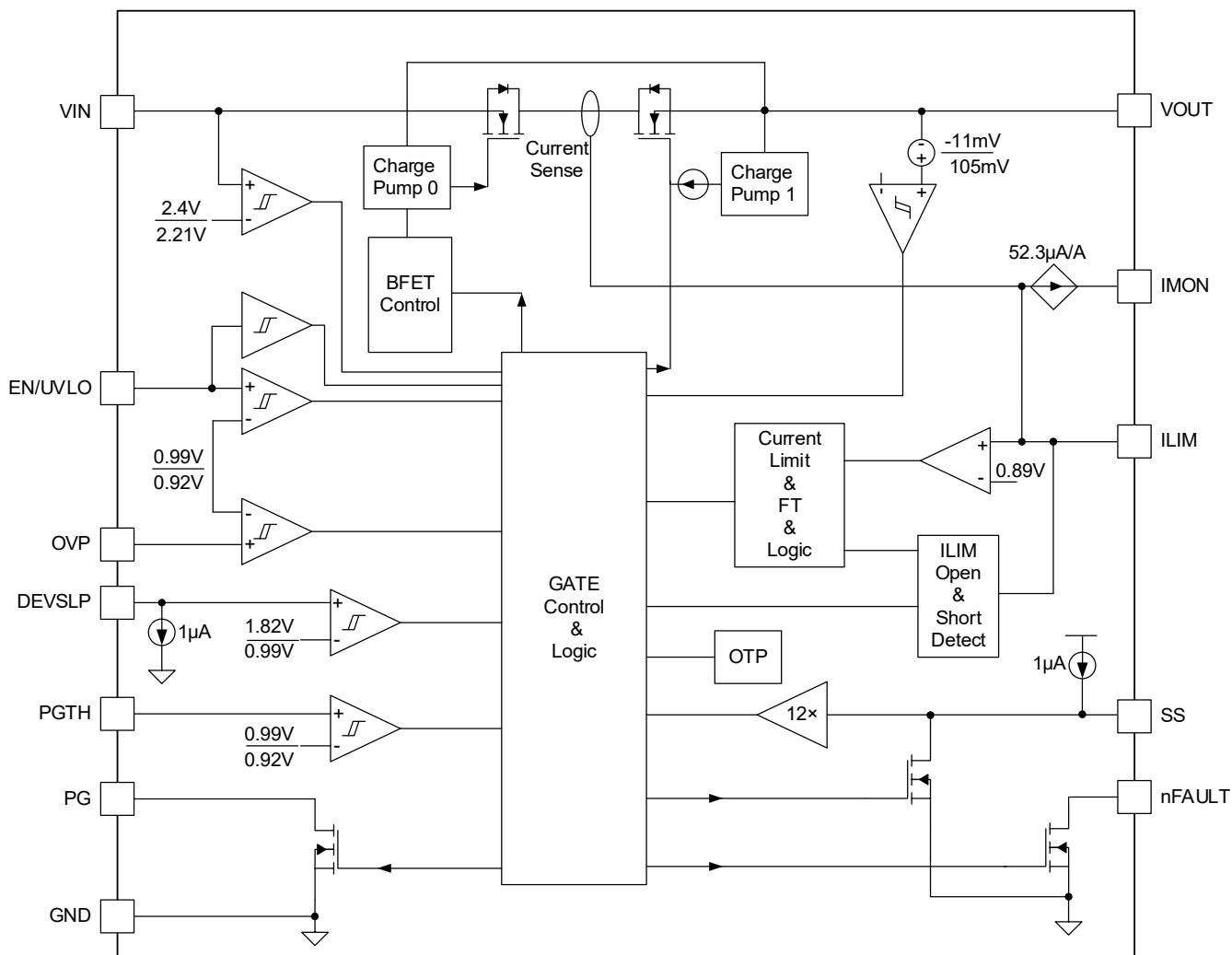
Figure 2. Block Diagram-SGM2535A/AL
