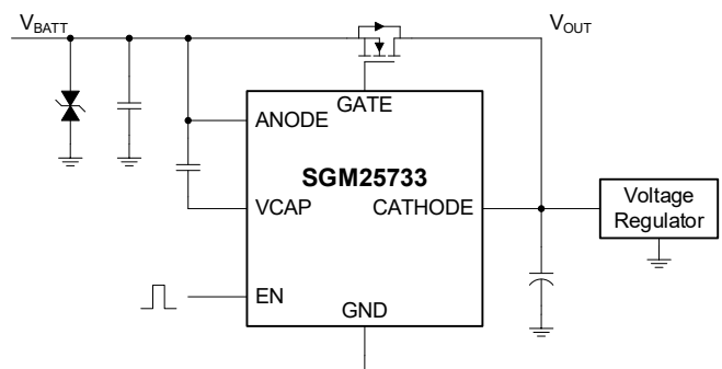
Figure 1. Application Schematic
