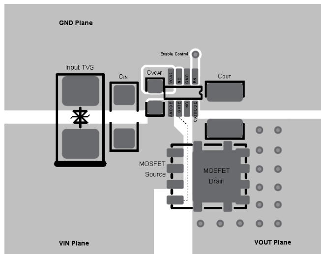
Figure 11. TSOT-23-8 Layout Example
