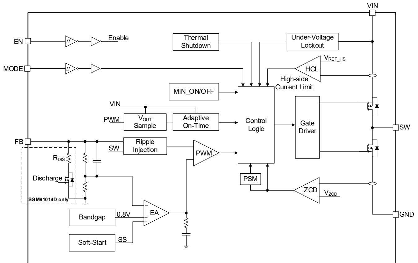
Figure 2. Block Diagram
