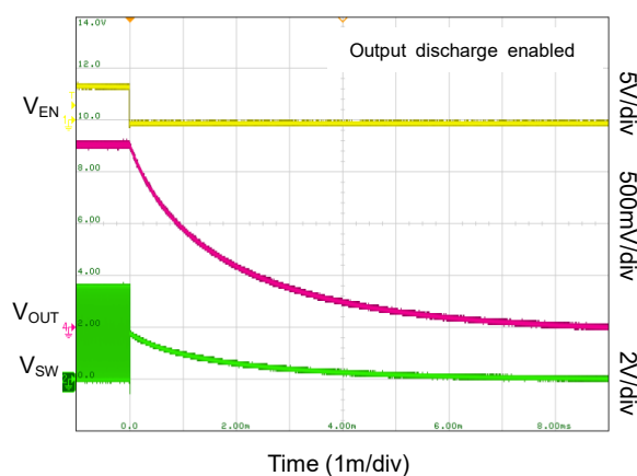
Shutdown (No Load, PWM Mode)
