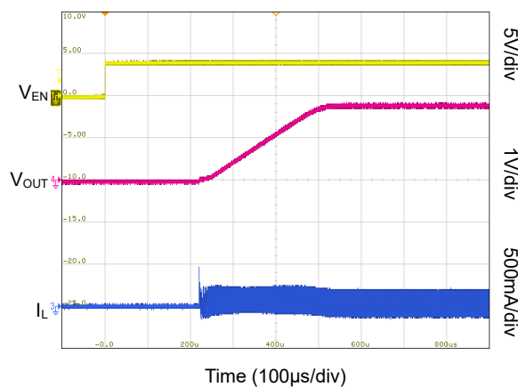
Startup (50 \Omega Load, PWM Mode)
