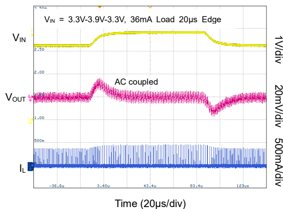
Line Transient (PFM Mode)
