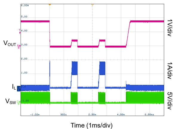
300mΩ Fault, Rapid Fault, Hiccup (PWM Mode)
