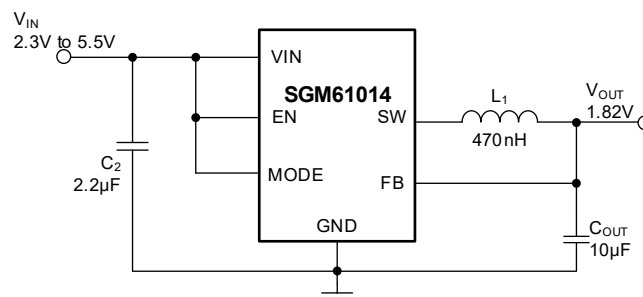
Figure 1. Simplified Schematic
