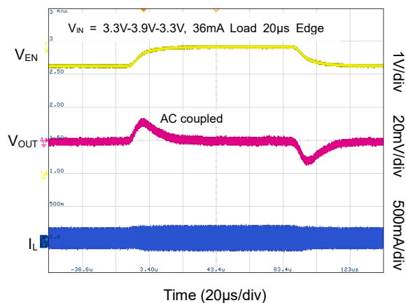
Line Transient (PWM Mode)
