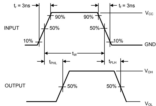
Figure 2. AC Waveforms
