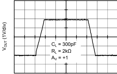
Time (5µs/div)
