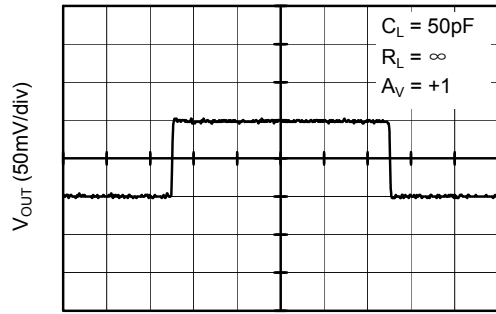
Time (5µs/div)
