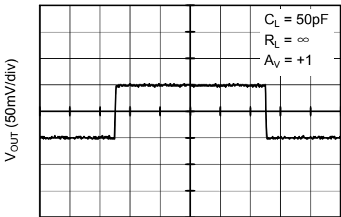
Time (5µs/div)
