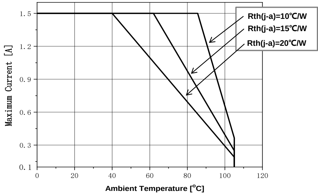
Fig 9. Maximum Forward Current vs. Ambient Temperature, T_j(max.)=150^{\circ}C
