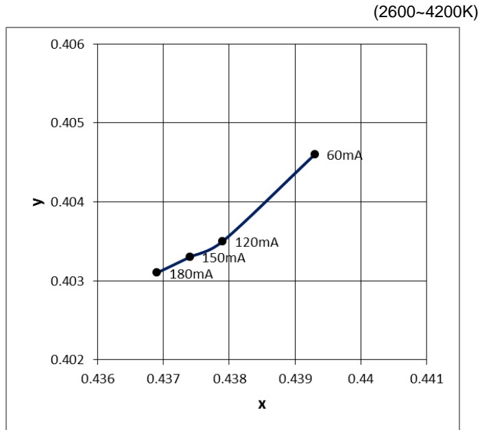
Fig 5. Forward Current vs. CIE X,Y Shift, T_j = 25^\circ\text{C}
