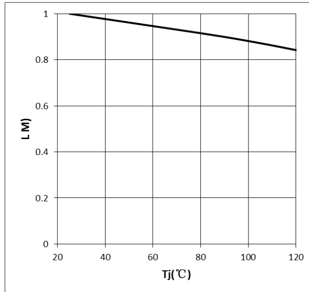
Fig 6. Junction Temperature vs. Relative Luminous Intensity, I_F=65\text{mA}
