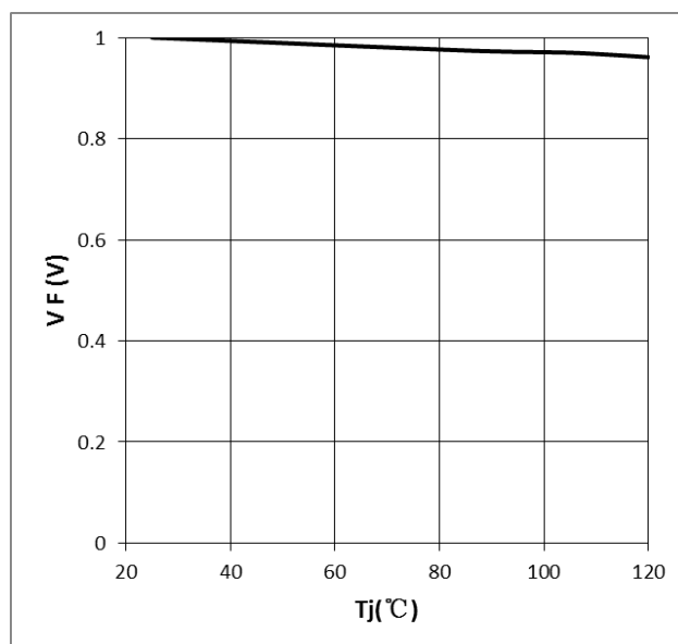
Fig 7. Junction Temperature vs. Relative Forward Voltage, I_F=65\text{mA}
