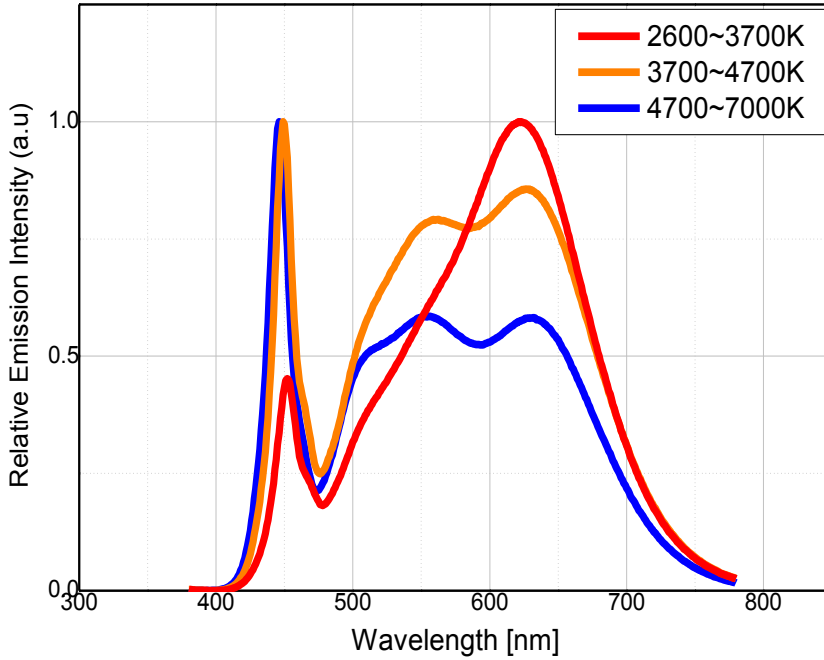
Fig 1. Color Spectrum, T_j = 25^\circ\text{C} , I_F = 120\text{mA}
