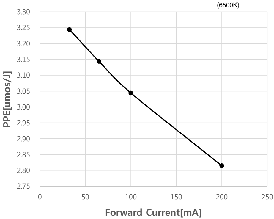
Fig 11. Forward Current vs. Photosynthetic Photon Energy , T_j = 25^\circ\text{C}
