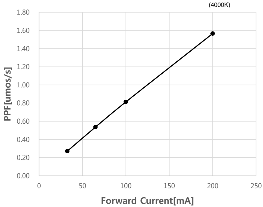
Fig 10. Forward Current vs. Photosynthetic Photon Flux, T_j = 25^\circ\text{C}
