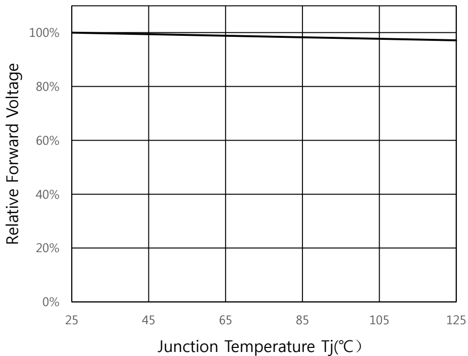
Fig 7. Junction Temperature vs. Relative Forward Voltage, I_F=120\text{mA}
