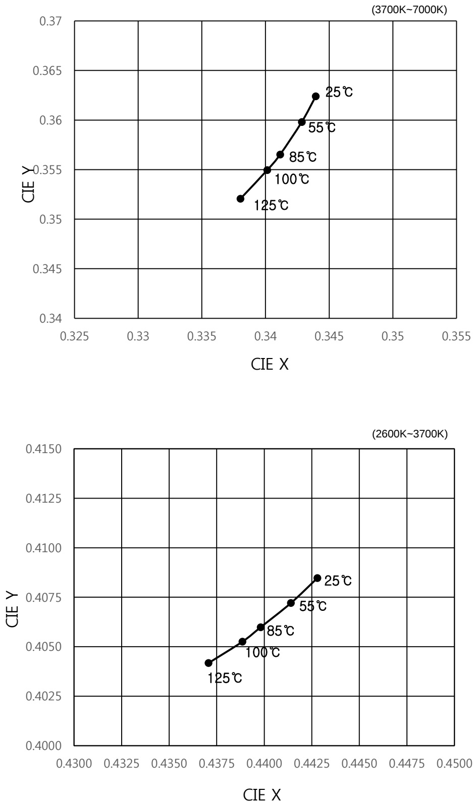
Fig 8. Chromaticity Coordinate vs. Junction Temperature, I_F=120\text{mA}
