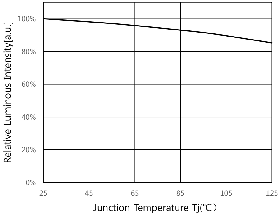
Fig 6. Junction Temperature vs. Relative Luminous Flux, I_F=120\text{mA}
