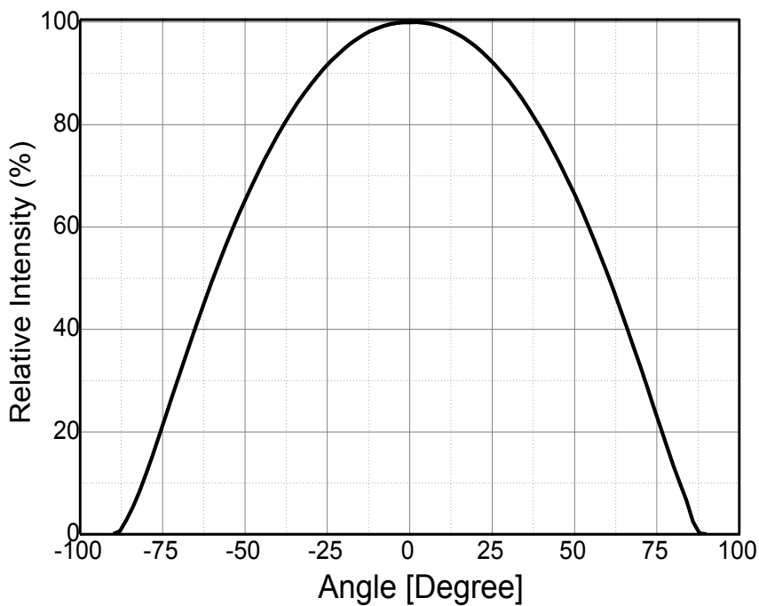
Fig 2. Radiant Pattern, T_j = 25^{\circ}\text{C} , I_F = 120\text{mA}
