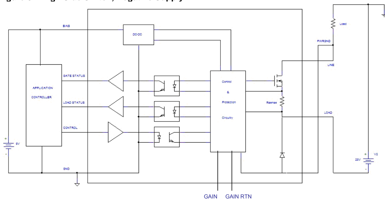
Figure 9 – Low Side Switch, Negative Supply
