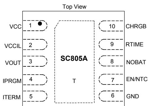
MLP-10 3mm x 3mm 10 Lead
