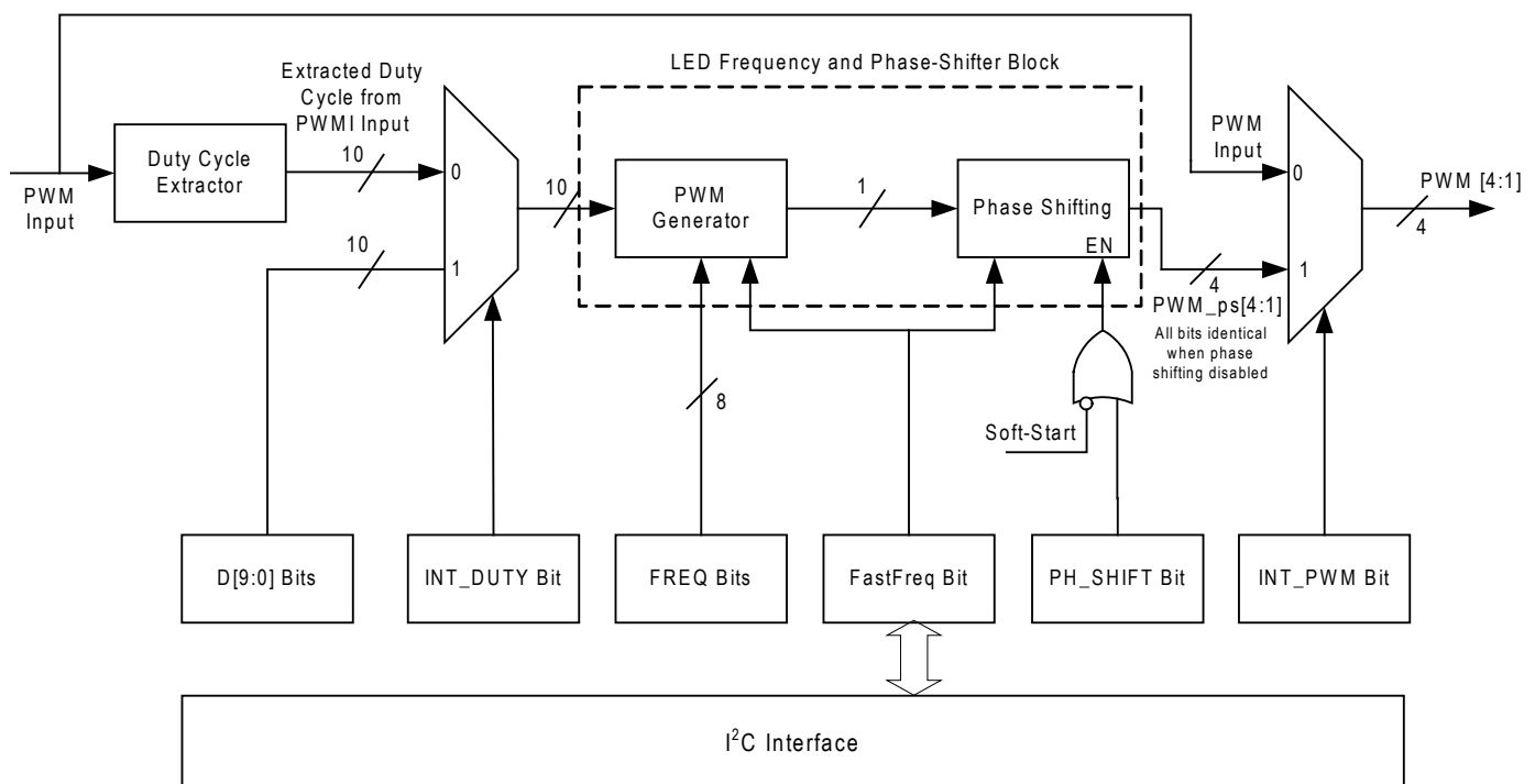
Figure 1— I 2 C Control Method
