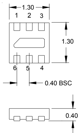
Nominal Dimensions (mm) (SLP1313P6T Bottom View)
