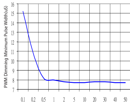
PWM Dimming Minimum Pulse Width vs. PWM Dimming Frequency
