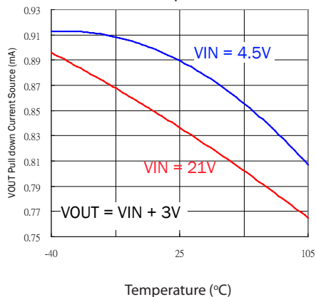
VOOUT Pull Down Current Source vs. Temperature
