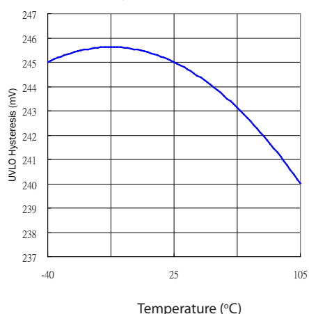
UVLO Hysteresis vs. Temperature
