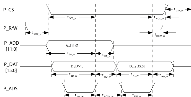
Figure 4-8: External Timing for Auto-Increment Write Cycle
