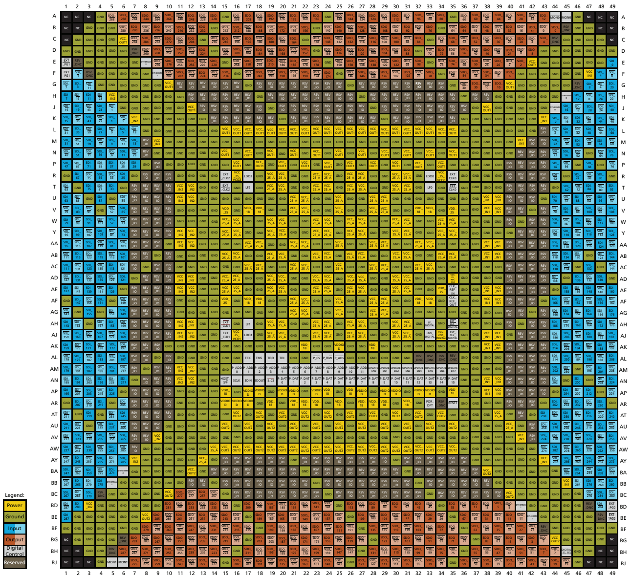
Figure 1-1: GX3202 Ball Assignment Overview (Top View)
