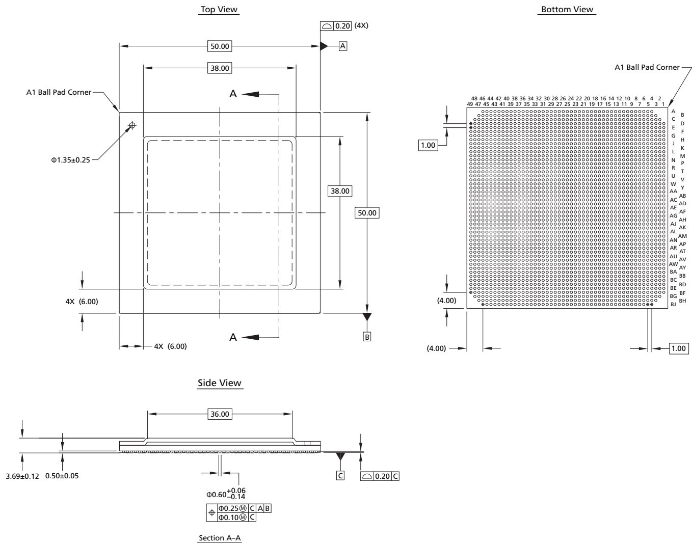
Figure 6-1: Package Dimensions
