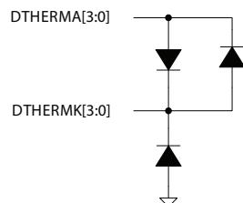
Figure 4-3: Temperature Sensors
