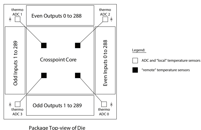
Figure 4-4: Map of Thermometer ADC Positions on Die
