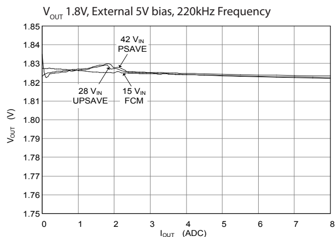
Load Regulation
