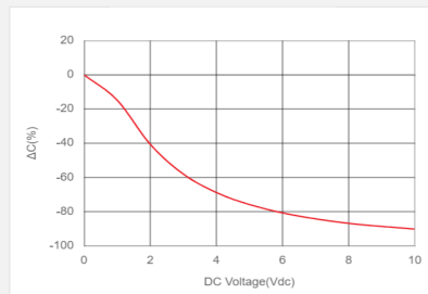
DC Bias Characteristics LCR meter, 1kHz, 0.5Vrms
