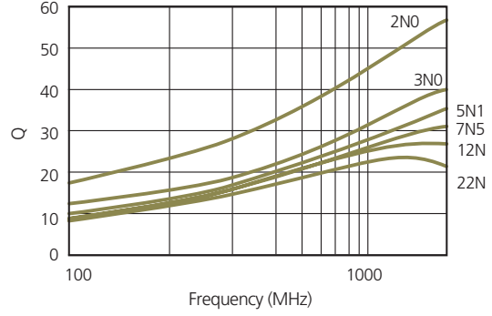
Q CHARACTERISTIC
