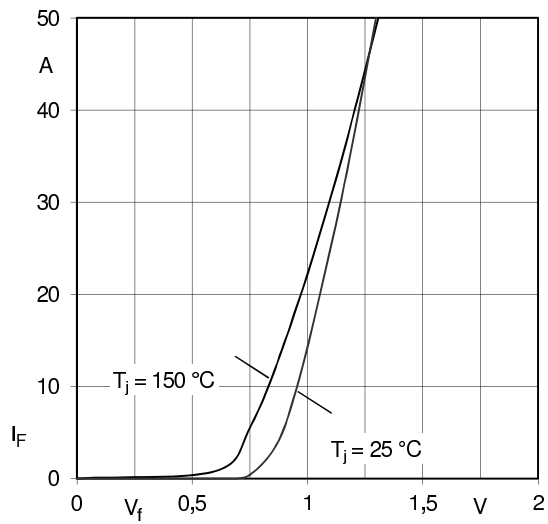
Fig. 7: Typ. input bridge forward characteristic
