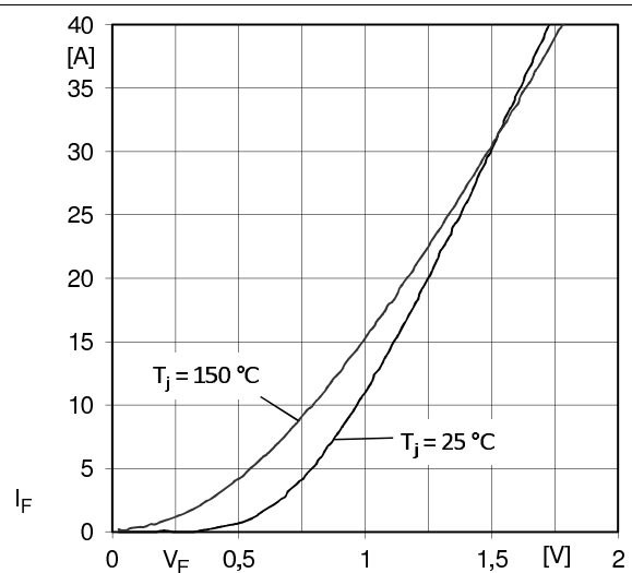
Fig. 6: Typ. freewheeling diode forward characteristic
