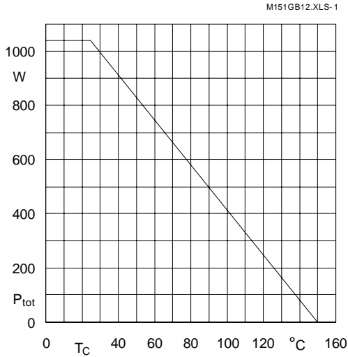
Fig. 1 Rated power dissipation P_{tot} = f(T_C)
