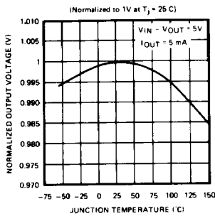
Output Voltage
