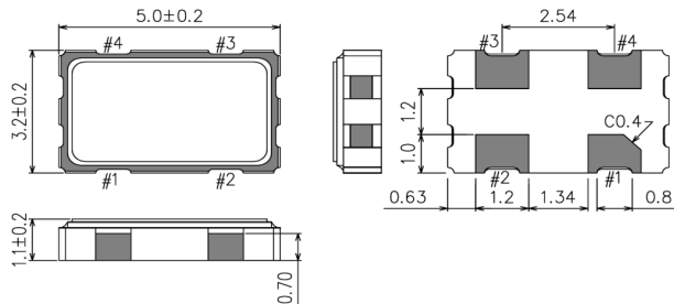
SG5032CAN
