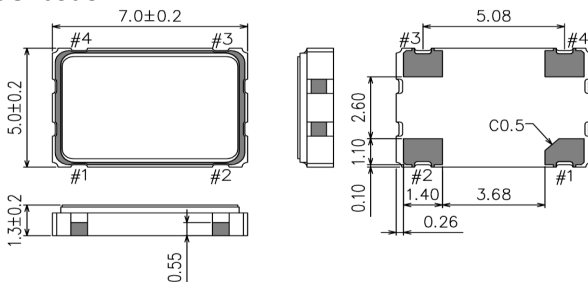
SG7050CAN
