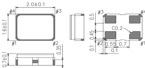
SG2016CAN
