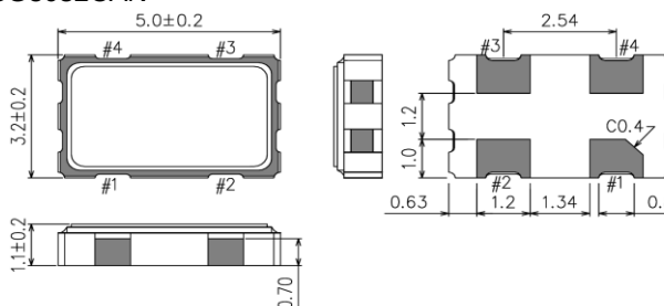
SG5032CAN
