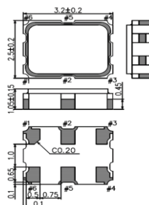
SG3225EEN
