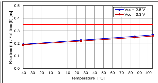
Fall Time
