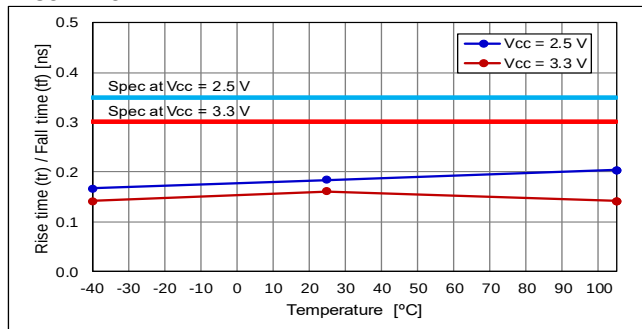
Rise Time
