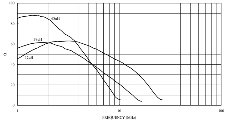
Q vs. FREQUENCY CHARACTERISTICS
