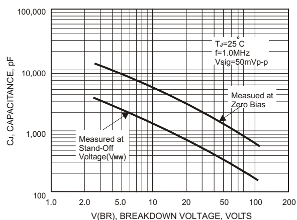
FIG.4-TYPICAL JUNCTION CAPACITANCE
