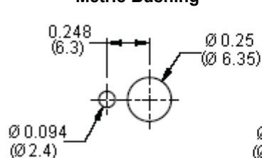
Metric Bushing
