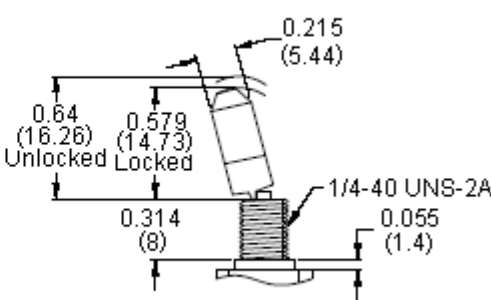
TL2B25
