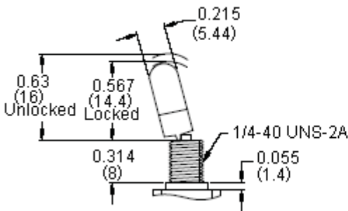
TL1B25
