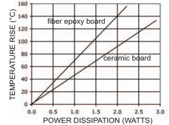
POWER DERATING
