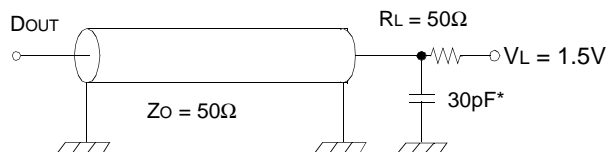
Output Loads(A)
