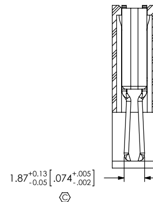
SECTION "B"-"B" SCALE 3:1
