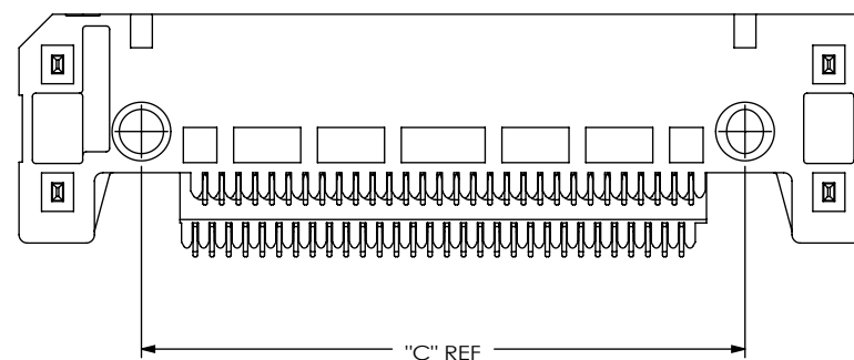
FIG 2 (ERF5-030-01-X-D-RA-FL-TR SHOWN) (NOT TOOLED) (SAME AS FIG 1, EXCEPT AS SHOWN)
