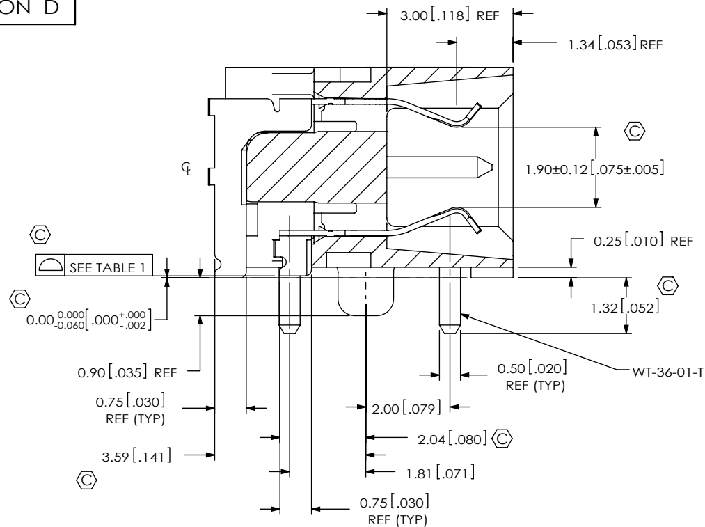
SECTION "A"-"A" SCALE 8 : 1
