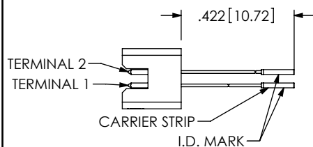
IN-PROCESS 1 (ORIENT I.D. MARK AS SHOWN) (FOR -RA OPTION ONLY)
