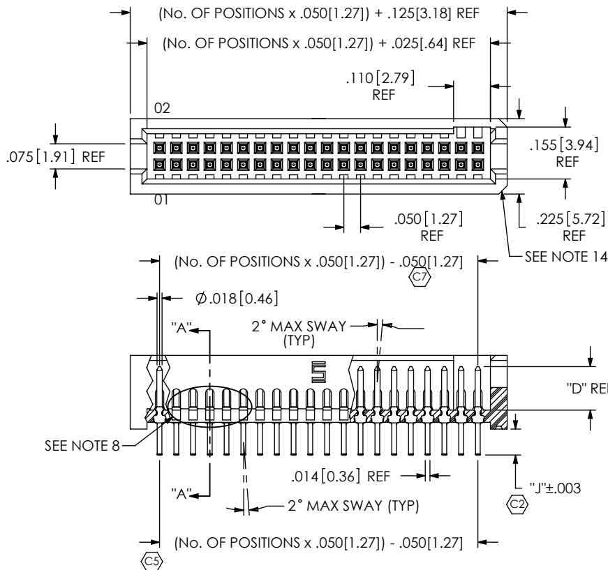
FIGURE 1 THROUGH HOLE -01, -03, -11, -13, -21, -23, -31
