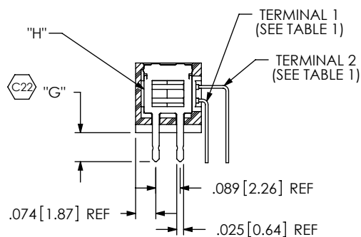
SECTION "J"-"J"
