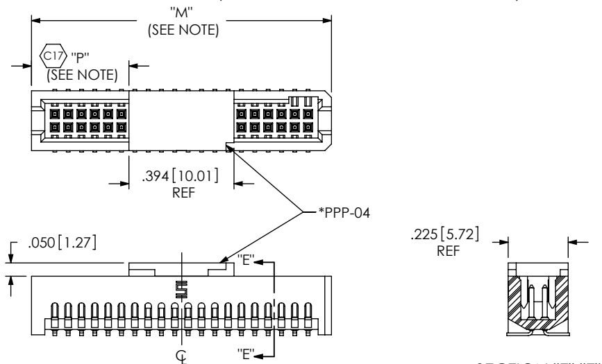
SECTION "E"-"E"
