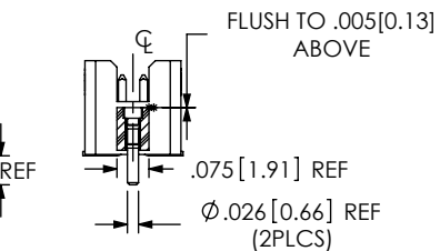
SECTION "K"-"K"
