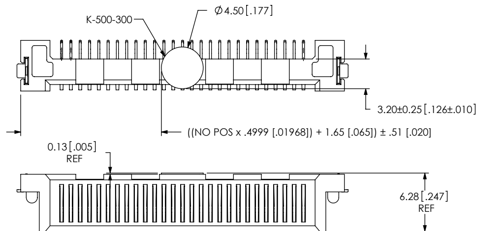
FIG. 2 SAL1-127-01-XX-S-A-K SHOWN SAME AS FIG. 1 EXCEPT AS SHOWN
