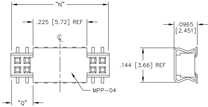
FIG. 3 -P: PICK & PLACE PAD AVAILABLE ON POSITIONS 7 THRU 50 ONLY
