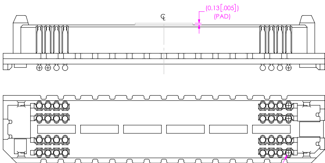
FIG 4 ADM6-30-01.5-XXX-4-X-XR SHOWN (SAME AS FIG1, EXCEPT AS SHOWN) (SOLDER BALL OPTION) (SOME CENTER FEATURES REMOVED FOR CLARITY)
