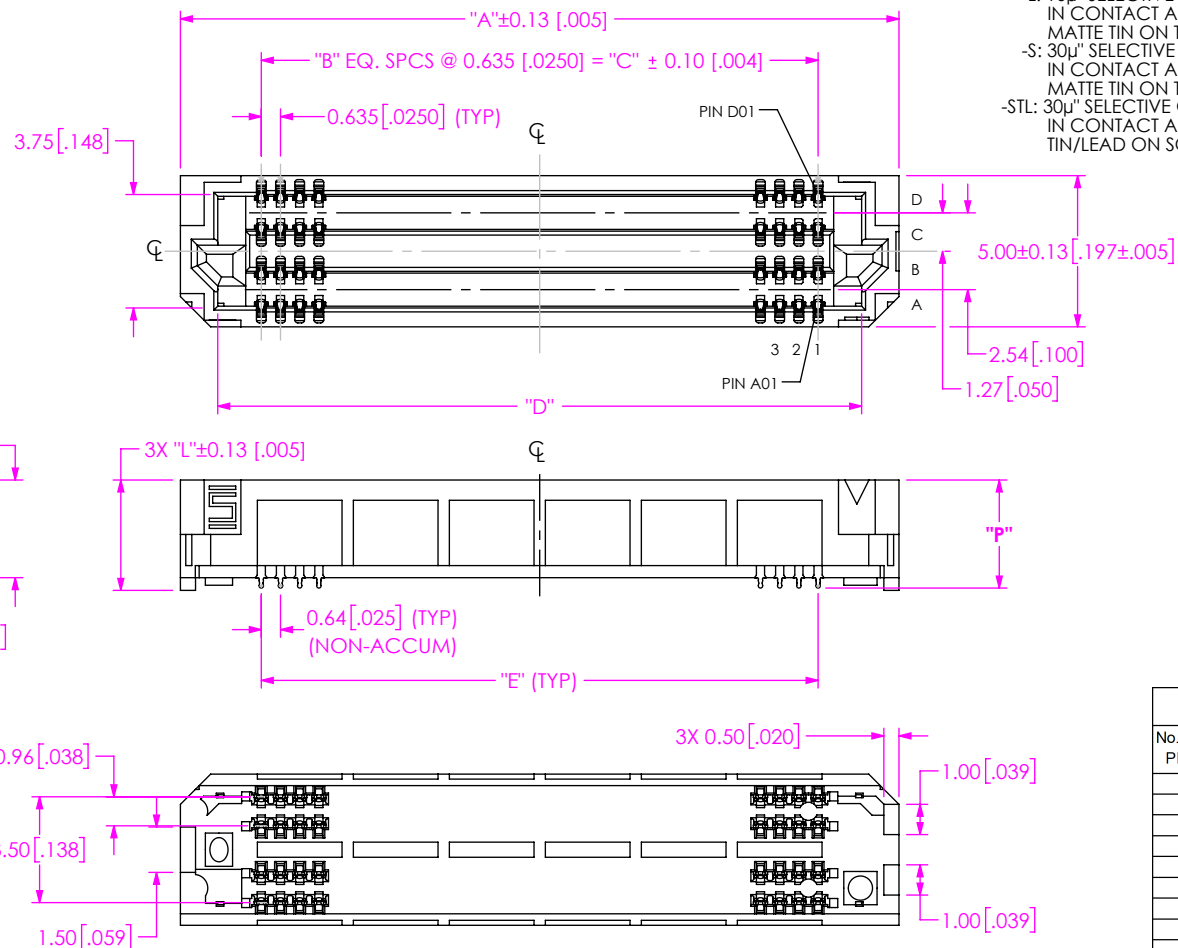
FIG 1 ADF6-30-03.5-XXX-4-0-XR SHOWN (SOME CENTER FEATURES REMOVED FOR CLARITY)
