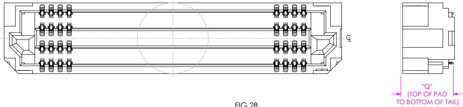
FIG 2B ADF6-30-03.5-XXX-4-0-XR SHOWN (COLUMN OPTION) (SOME CENTER FEATURES REMOVED FOR CLARITY) (SAME AS FIG 2A, EXCEPT AS SHOWN)
