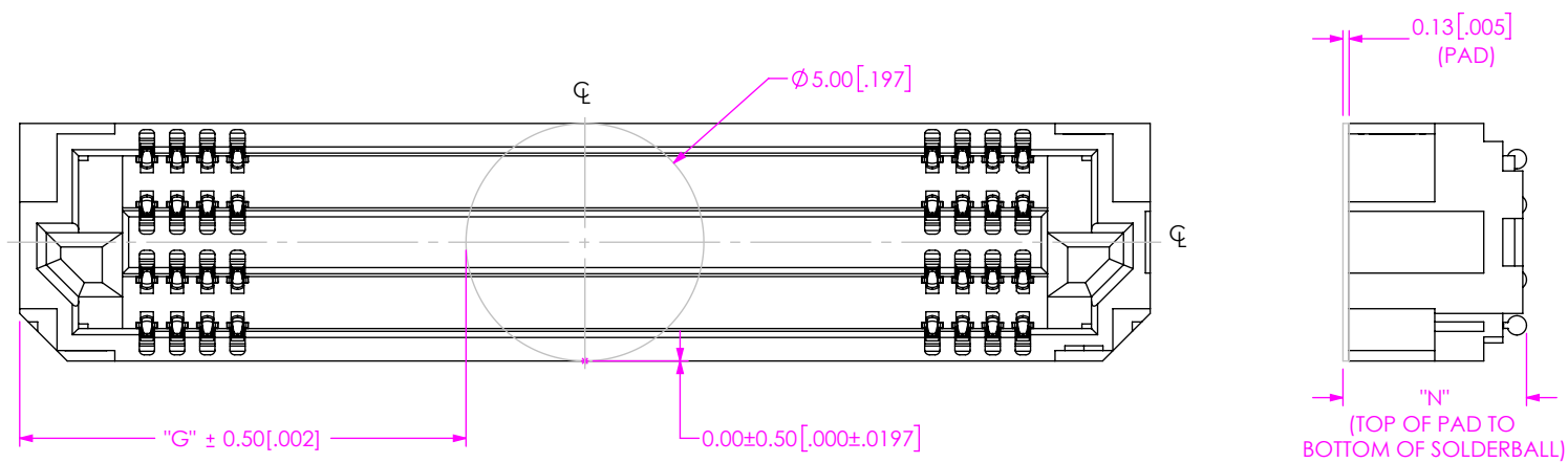
FIG 2A POLYIMIDE PAD ADF6-30-03.5-XXX-4-X-XR SHOWN (SOLDERBALL OPTION) (SOME CENTER FEATURES REMOVED FOR CLARITY)
