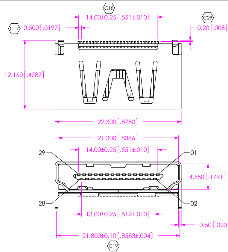
FIG 7 HDMR-29-01-X-SM-PF SHOWN (DIFFERENT AS SHOWN, OTHERWISE SAME AS FIG 6)
