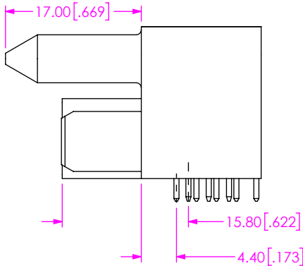
FIG 10 ET60T-D04-3-08-A04-X-R1-T SHOWN (DIFFERENT AS SHOWN, OTHERWISE SAME AS FIG 1)
