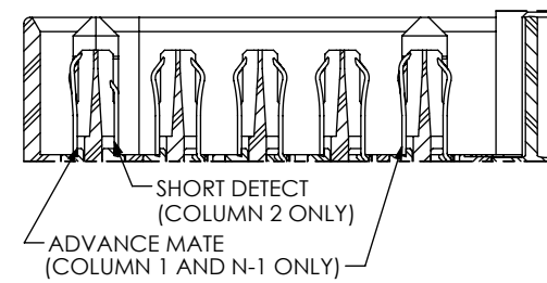
SECTION "C"-"C" SCALE 2.5 : 1
