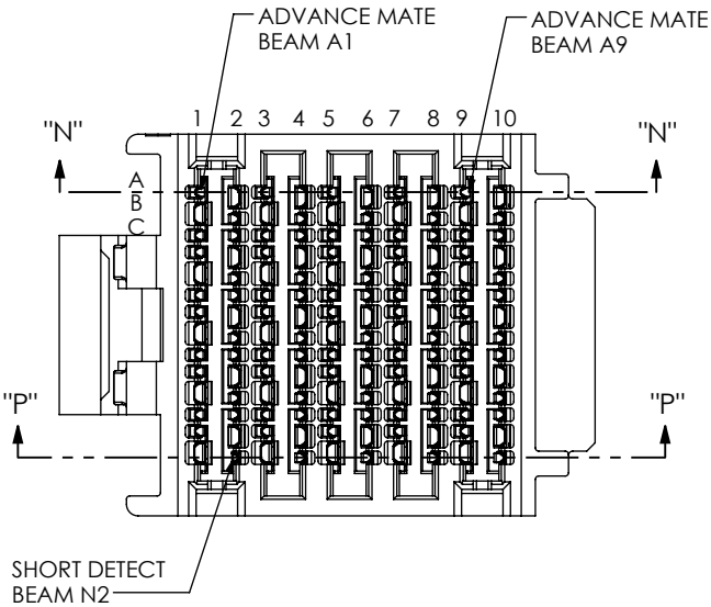
FIG 5 ADVANCED MATE AND SHORT DETECT EBCF-X-4-10-V-2 SHOWN (DIFFERENT AS SHOWN, OTHERWISE SAME AS FIG 3 & 4) (NOT TOOLED)
