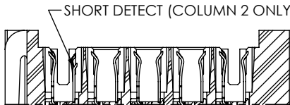
SECTION "P"-"P" SCALE 2 : 1
