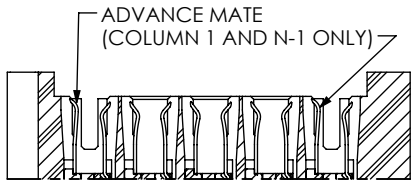
SECTION "N"-"N" SCALE 2 : 1
