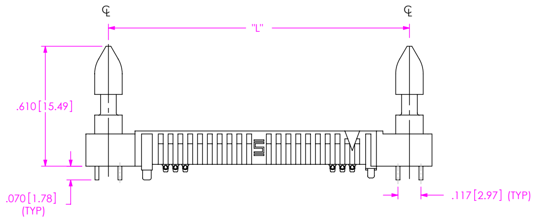
FIG 4 LATCH POST OPTION (SEAF-20-5.0-X-06-1-K-XR SHOWN) (SOME CENTER FEATURES REMOVED FOR CLARITY) (DIFFERENT AS SHOWN, OTHERWISE SAME AS FIG 1) (LATCH POST OPTION REQUIRED FOR SEAC MATE ONLY) (ONLY AVAILABLE WITH -5.0 LEAD STYLE -04, -06, -08 & -10 ROW)
