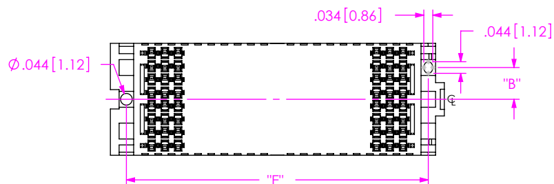
FIG 1 -08: 8 ROW (SEAFC-20-5.0-X-08-1-N-K-XR SHOWN) (SOME CENTER FEATURES REMOVED FOR CLARITY)
