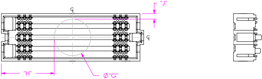
FIG 3 K-DOT (SEAFC-20-5.0-X-08-1-N-K-XR SHOWN) (DIFFERENT AS SHOWN, OTHERWISE SAME AS FIG 1) (SOME CENTER FEATURES REMOVED FOR CLARITY)
