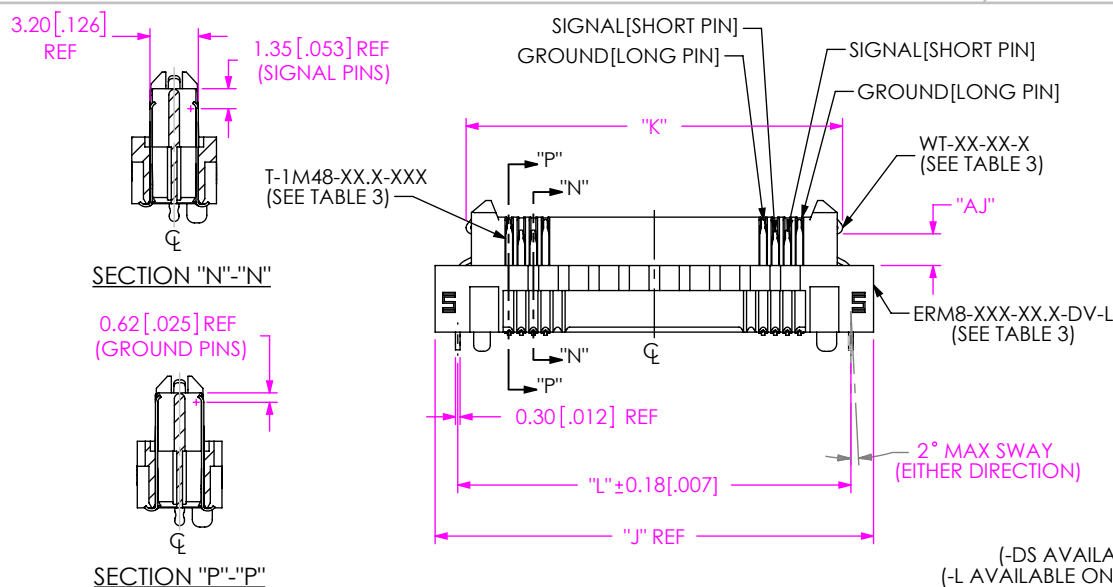
FIG 3 -DS WITH -L OPTION (-DS AVAILABLE ON -05.0 LEAD STYLE ONLY) (-L AVAILABLE ON -03.0, -05.0 & -09.0 LEAD STYLE ONLY) (ERM8-025-05.0-XXX-DV-DS-L SHOWN) (SAME AS FIG 1, EXCEPT AS SHOWN) (SOME CENTER FEATURES REMOVED FOR CLARITY)
