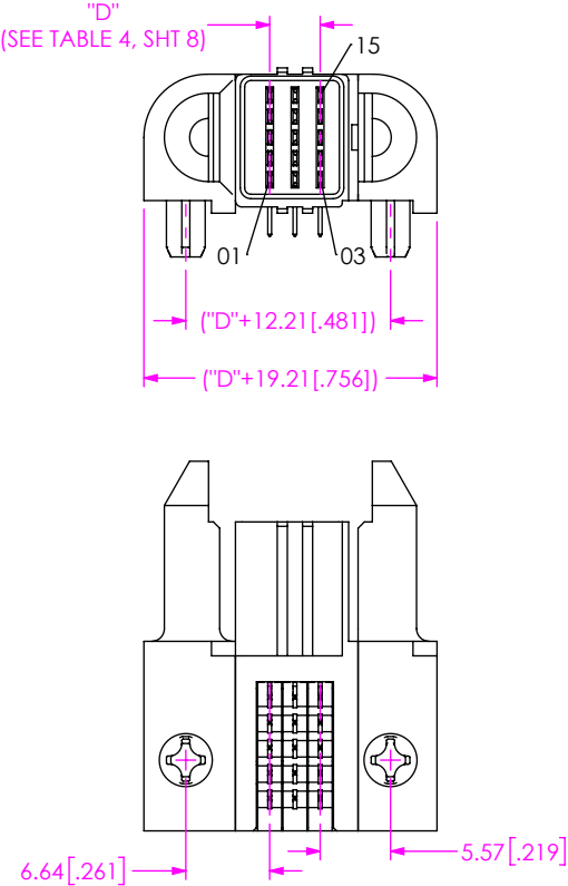
FIG 15 ET60T-000-5-03-000-X-RX-S SHOWN (DIFFERENT AS SHOWN, OTHERWISE SAME AS FIG 4)
