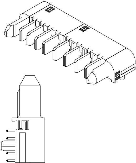
FIG 7 ET60T-D04-0-00-A04-X-R1-S SHOWN (DIFFERENT AS SHOWN, OTHERWISE SAME AS FIG 1)
