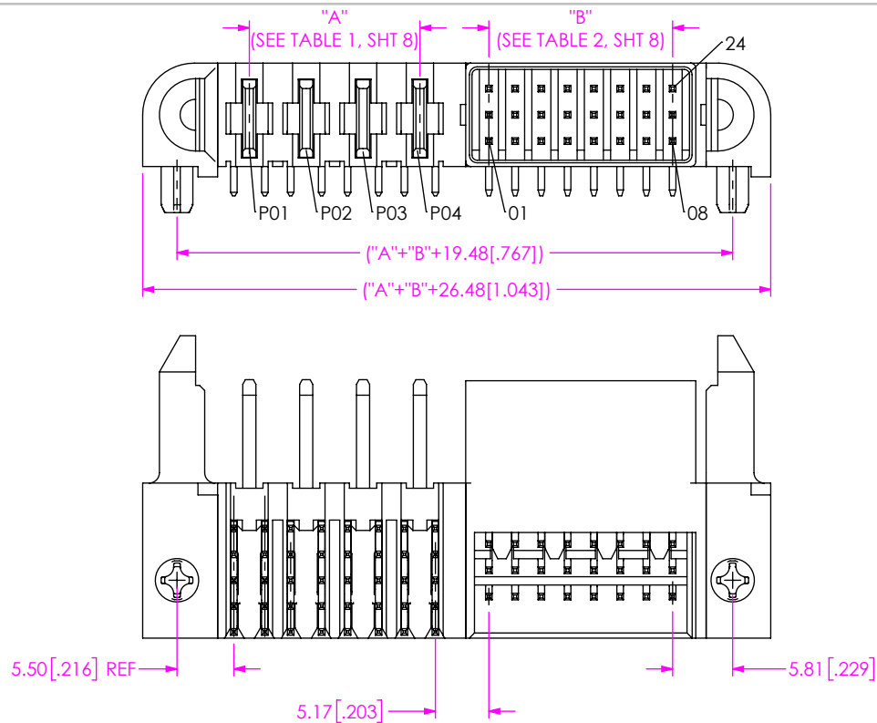
FIG 3 ET60T-D04-3-08-000-X-R1-S SHOWN (DIFFERENT AS SHOWN, OTHERWISE SAME AS FIG 1)
