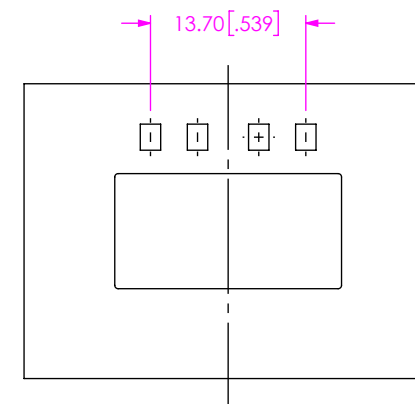
FIG 9 QSFP-C-1-X-S-LP-F WITH FQSFP-LP-04 SHOWN (4 LIGHTPIPES) (DIFFERENT AS SHOWN, OTHERWISE SAME AS FIG 8)
