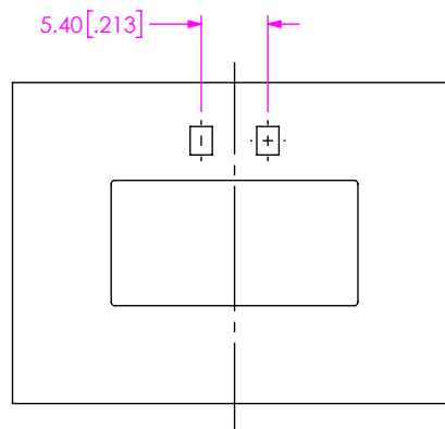
FIG 8 QSFP-C-1-X-S-LP-F WITH FQSFP-LP-02 SHOWN (2 LIGHTPIPES) (DIFFERENT AS SHOWN, OTHERWISE SAME AS FIG 7)
