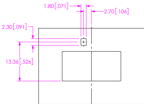
FIG 7 QSFP-C-1-X-S-LP-F WITH FQSFP-LP-01 SHOWN (1 LIGHTPIPE) (DIFFERENT AS SHOWN, OTHERWISE SAME AS FIG 6)
