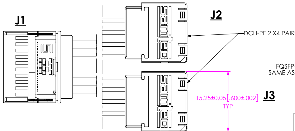
FIG 1 FQSFP-01-XX.X-L-PF-1 SHOWN
