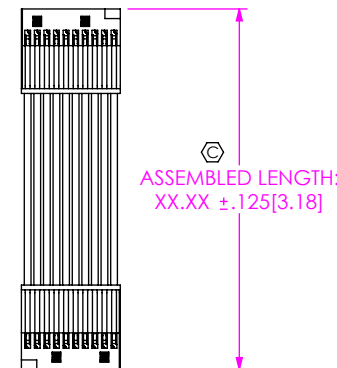
FIG 2 -D: DOUBLE END SFSD-10-28-XX-XX-XX-D-NUS SHOWN (SAME AS FIG 1, UNLESS OTHERWISE STATED)
