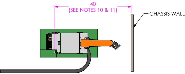
-7 FIBER TYPE RECOMMENDED CABLE ESCAPE CLEARANCE
