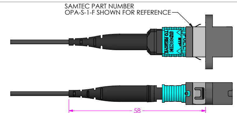
-7/-8 FIBER TYPE, -01/-02 END OPTION MATED WITH BULKHEAD DUST CAPS/PLUGS NOT SHOWN FOR CLARITY
