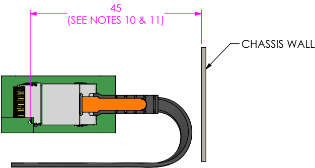
-5 FIBER TYPE RECOMMENDED CABLE ESCAPE CLEARANCE
