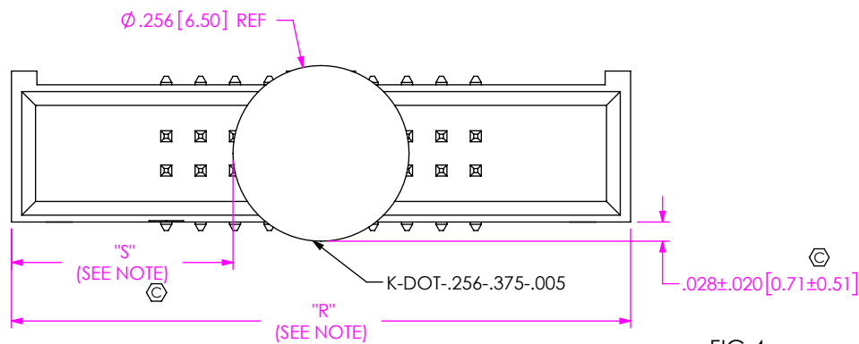
NOTE: "R" = USED MEASURED DIMENSION (REF) "S" = {("R" -.256[6.50])/2} ±0.020[0.51] FIG 4 (ESHF-110-01-X-D-SM-K SHOWN) (SAME AS FIG 1, DIFFERENT AS SHOWN)
