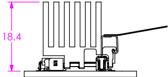
-2 PIN-FIN HEAT SINK
