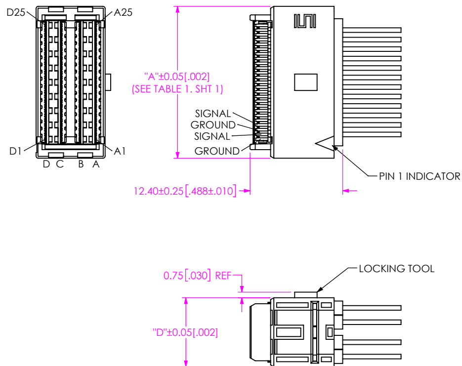
FIG 5 ARP6-SE-025-04-XX.X-X-T-X END 1 SHOWN
