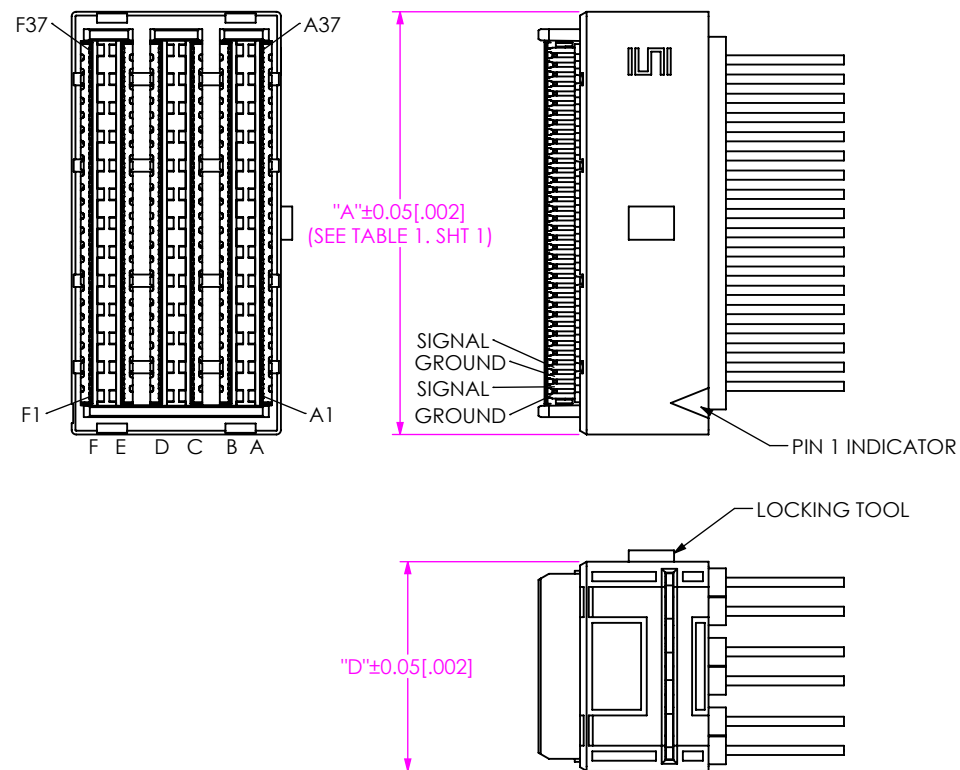
FIG 6 ARP6-SE-037-06-XX.X-X-T-X END 1 SHOWN (DIFFERENT AS SHOWN, OTHERWISE SAME AS FIG 5)
