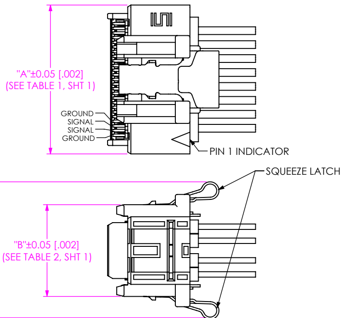
FIG 3 ARP6-DP-025-04-XX.X-X-L-X END 1 SHOWN (DIFFERENT AS SHOWN, OTHERWISE SAME AS FIG 1)
