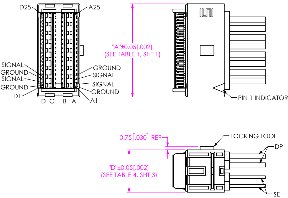
FIG 7 ARP6-DS-025-04-XX.X-X-T-X END 1 SHOWN
